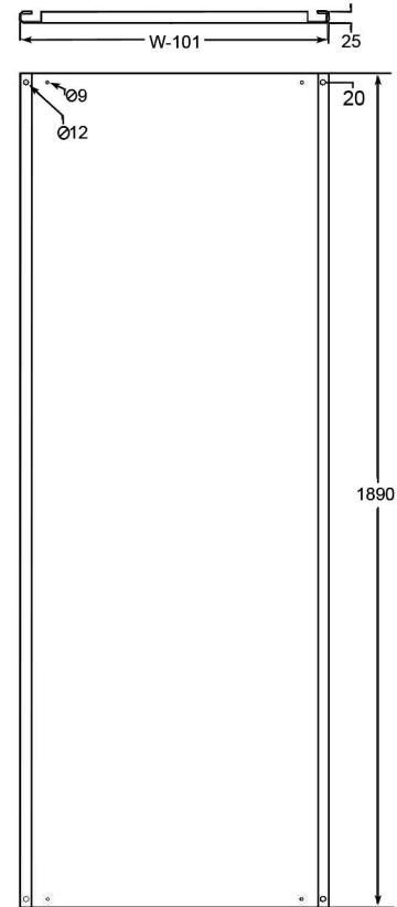
MOUNTING PLATE
