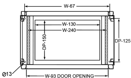
SECTIONAL TOP VIEW
