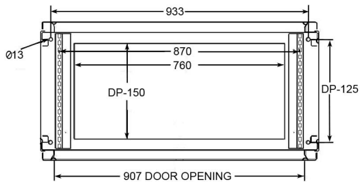
SECTIONAL TOP VIEW
