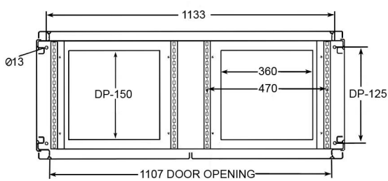
SECTIONAL TOP VIEW
