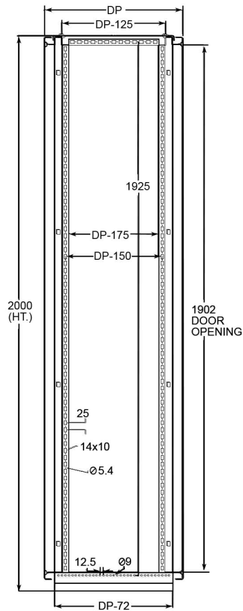
SECTIONAL SIDE VIEW
