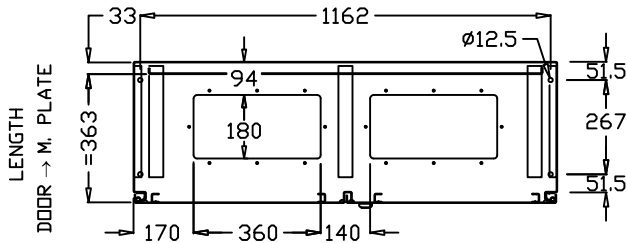
SECTIONAL BOTTOM VIEW 'A-A'
