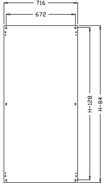
MOUNTING PLATE
